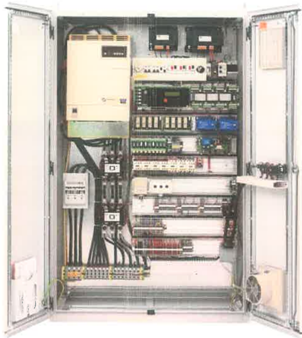
Microprocessor Controller
