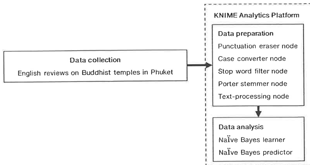
Figure 3: Sentiment analysis process in the KNIME Analytics Platform
